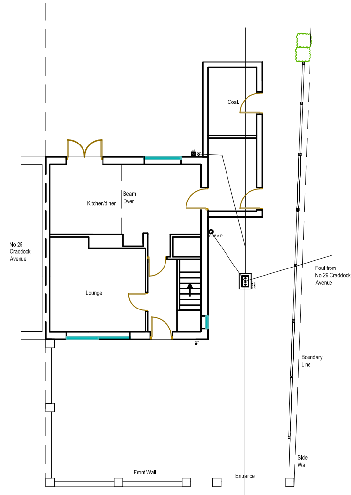
GROUND FLOOR PLAN AS EXISTING (1:100)
