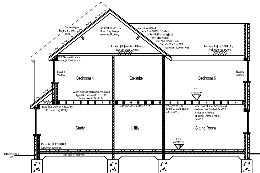
SECTION (1:50)
