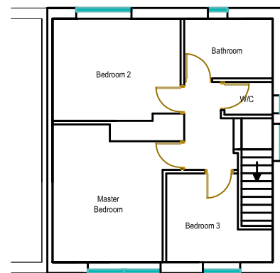
FIRST FLOOR PLAN AS EXISTING (1:100)
