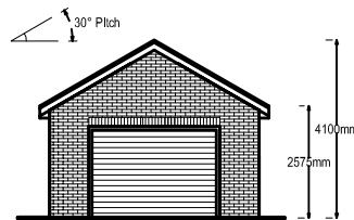
FRONT ELEVATION AS PROPOSED (1:100)
