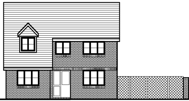
FRONT ELEVATION AS EXISTING (1:100)
