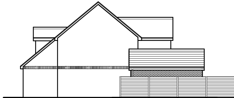
SIDE ELEVATION AS PROPOSED (1:100)
