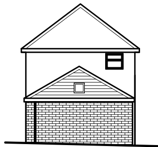
SIDE ELEVATION AS PROPOSED (1:100)
