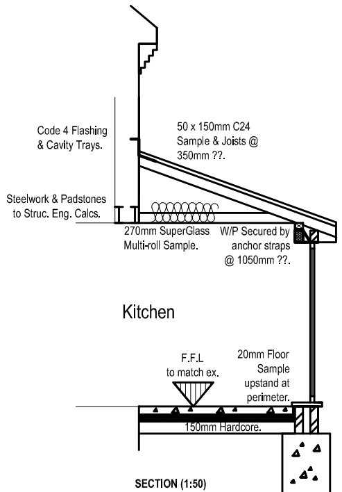
SECTION (1:50)
