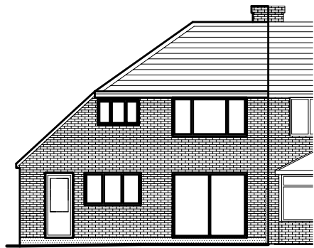
REAR ELEVATION AS EXISTING (1:100)
