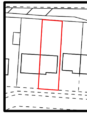
PLAN VIEW (1:500)
