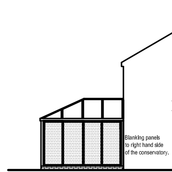
SIDE ELEVATION AS PROPOSED (1:100)
