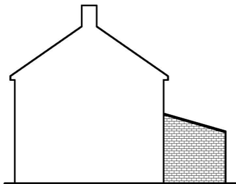
SIDE ELEVATION AS EXISTING (1:100)
