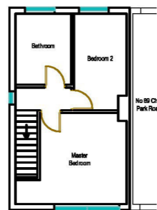
FIRST FLOOR PLAN AS EXISTING (1:100)
