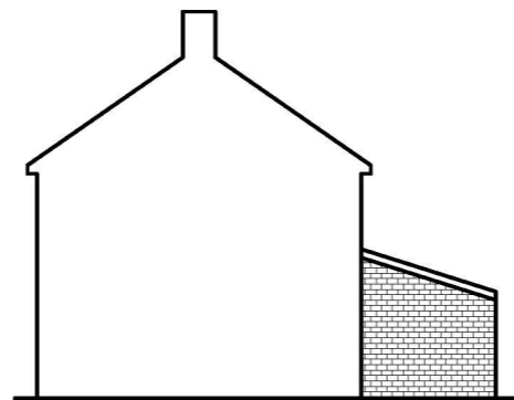
SIDE ELEVATION AS PROPOSED (1:100)
