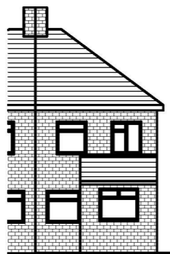
REAR ELEVATION AS EXISTING (1:100)
