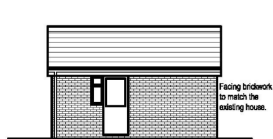
SIDE ELEVATION AS PROPOSED (1:100)
