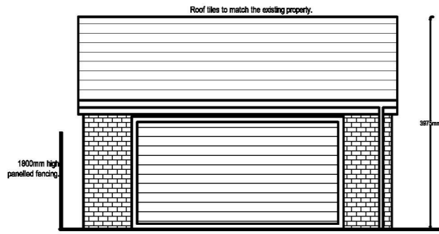
FRONT ELEVATION AS PROPOSED (1:50)
