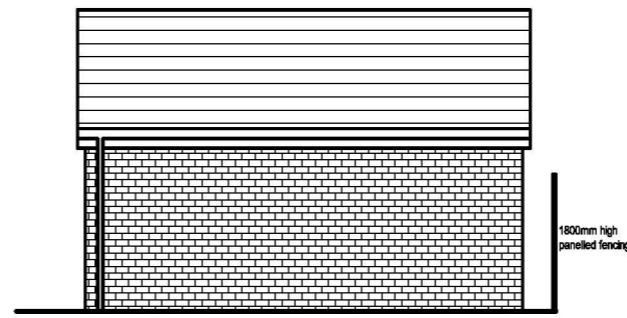
REAR ELEVATION AS PROPOSED (1:50)
