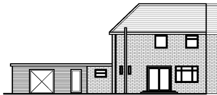
FRONT ELEVATION AS EXISTING (1:100)
