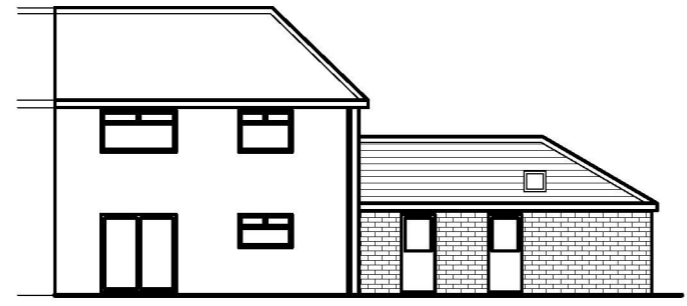
REAR ELEVATION AS PROPOSED (1:100)
