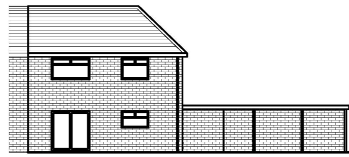
REAR ELEVATION AS EXISTING (1:100)
