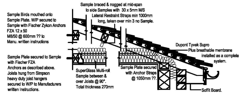
ROOF DETAIL (NTS)
